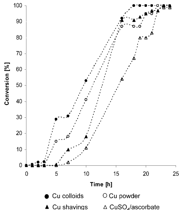
Figure 1. Time-resolved reaction profiles observed for the 1,3-cycloaddition of prop-2-yn-1-ol to benzyl azide using various copper catalytic systems. Reaction conditions are as in Table 1. All reactions were performed in duplicate (with error of \pm 2.3\% ).
