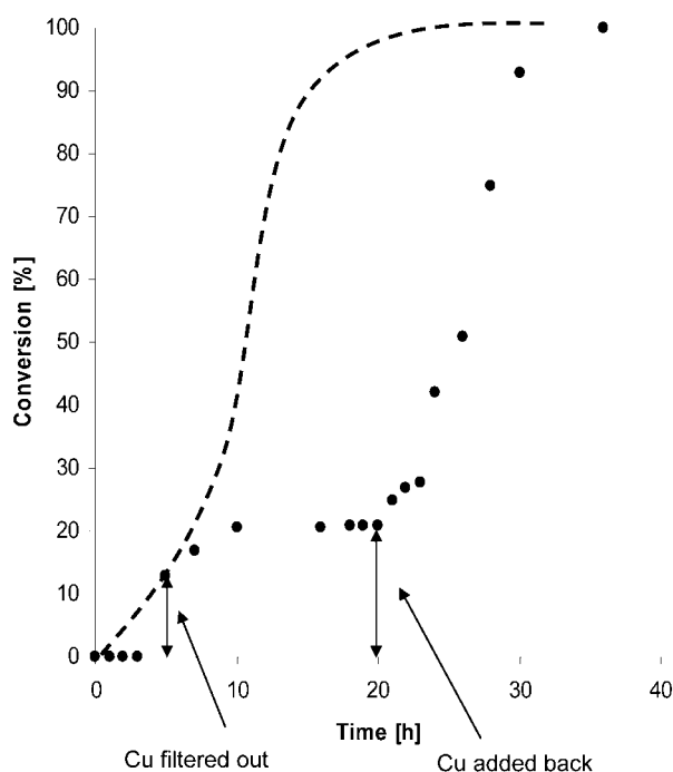
Figure 2. Time-resolved reaction profile observed for the 1,3-cycloaddition of prop-2-yn-1-ol and benzyl azide using Copper powder as catalyst. Reaction conditions are as in Table 1. '•' symbols represent the kinetic profile of the experiment filtering and adding back Cu powder. The broken line shows a control experiment without filtering of the copper catalyst.
