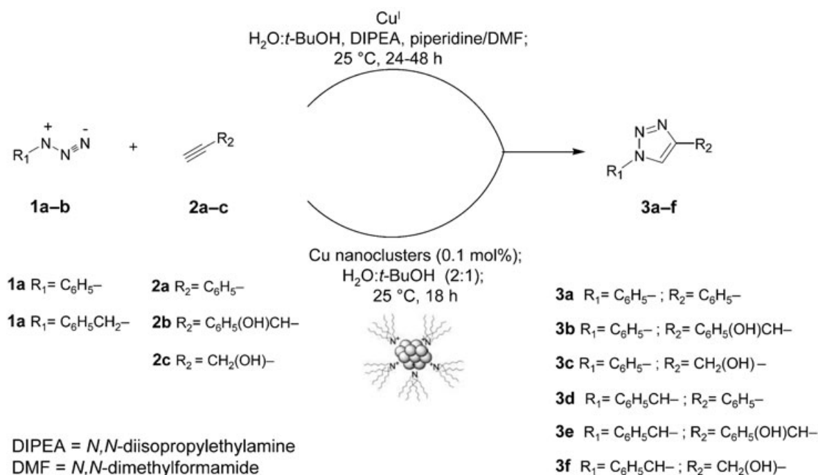
Scheme 1. Huisgen-type 1,3-cycloaddition of azides to terminal alkynes catalyzed by Cu(I) ions (top) and by Cu nanoclusters (bottom).
